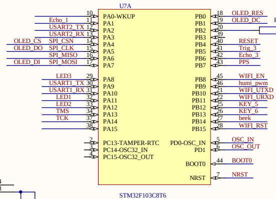
STM32F103C8T6
